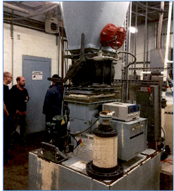
Photo 3-9 – Soda Ash Hopper, Dissolving Tank, and Metering Pumps
