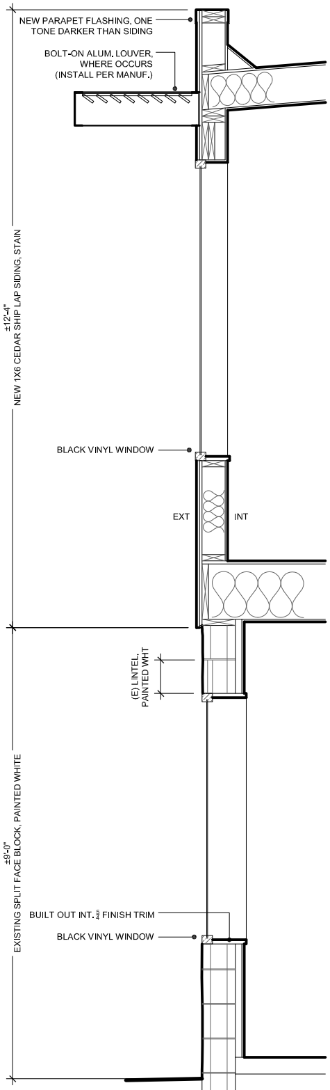
① BUILDING SECTION SCALE: 3/4" = 1' - 0"
