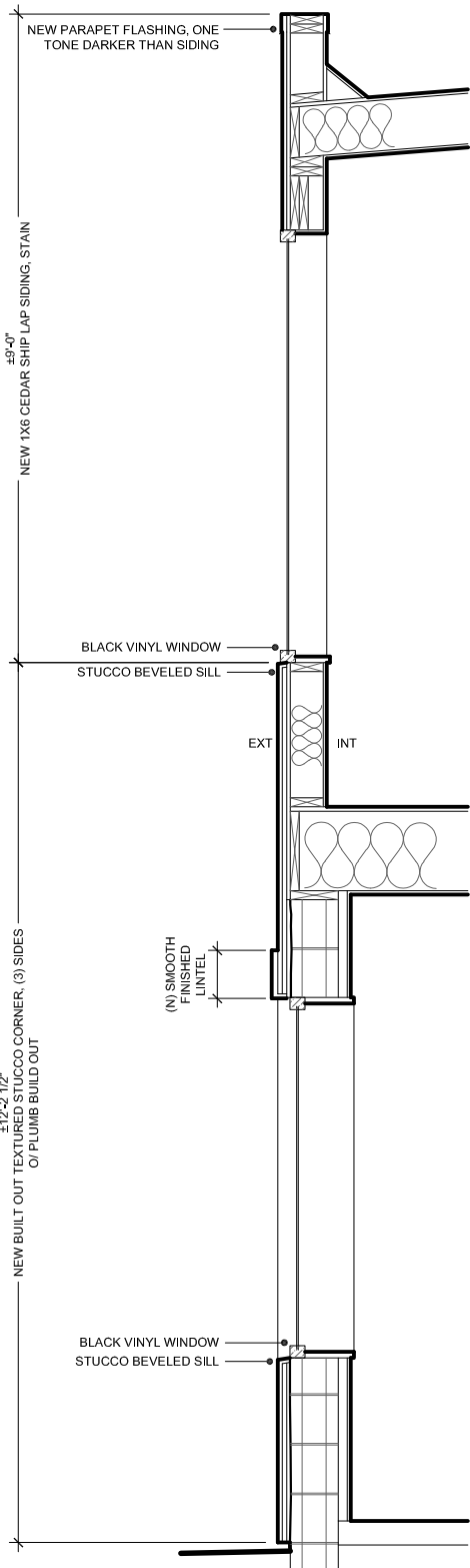
② BUILDING SECTION SCALE: 3/4" = 1' - 0"
