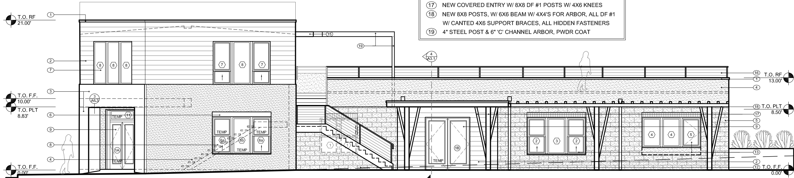
WEST ELEVATION
