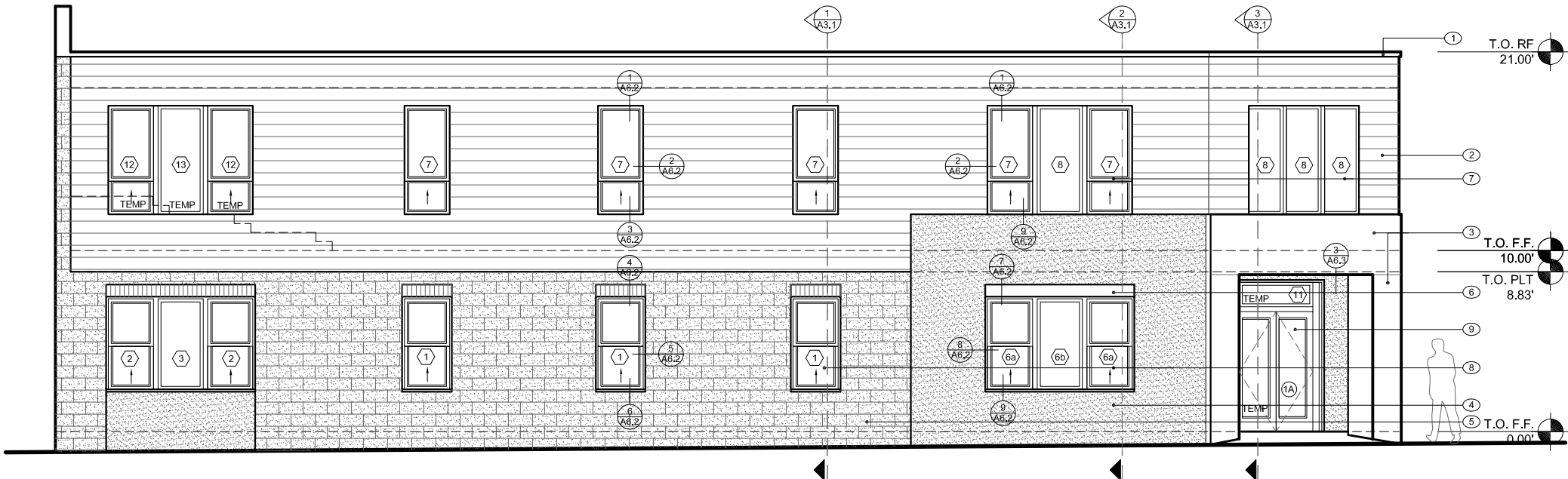
NORTH ELEVATION
