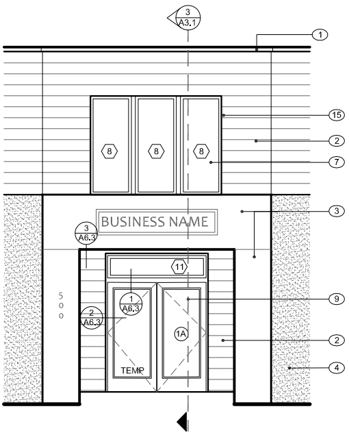
NW ELEVATION
