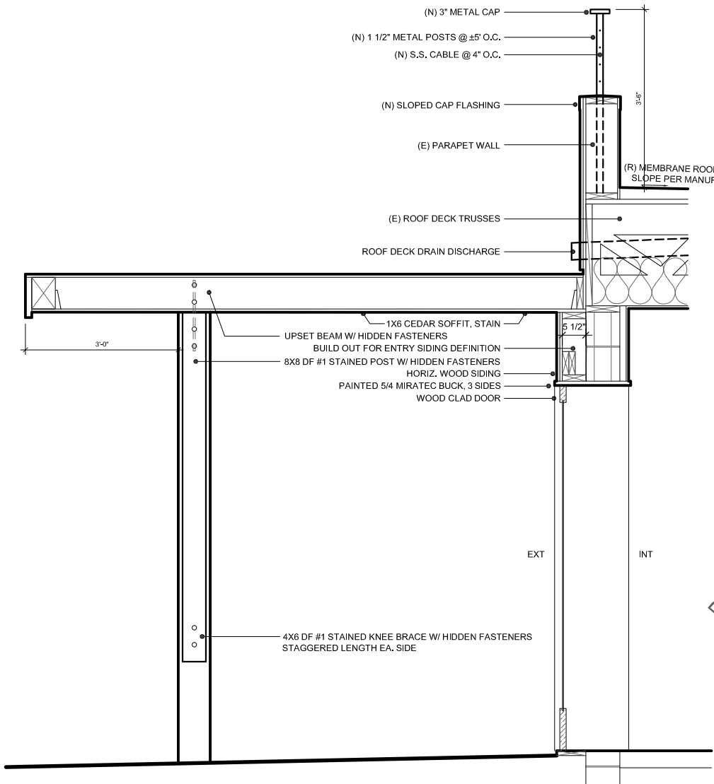
④ BUILDING SECTION SCALE: 3/4" = 1' - 0"
