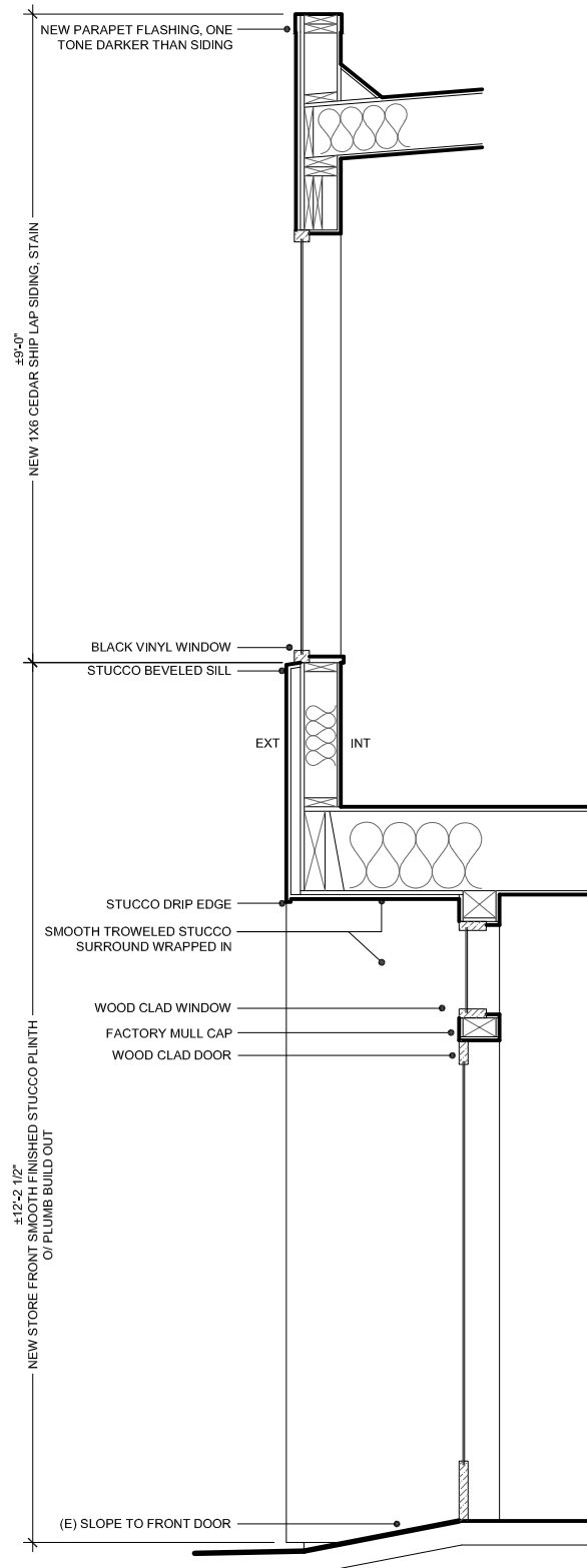
③ BUILDING SECTION SCALE: 3/4" = 1' - 0"
