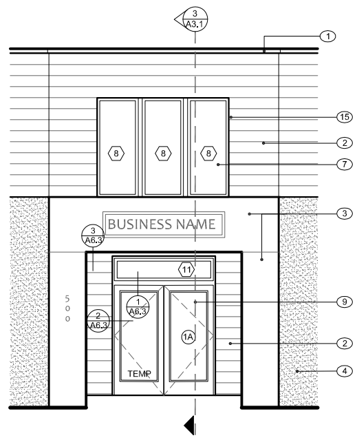
NW ELEVATION
