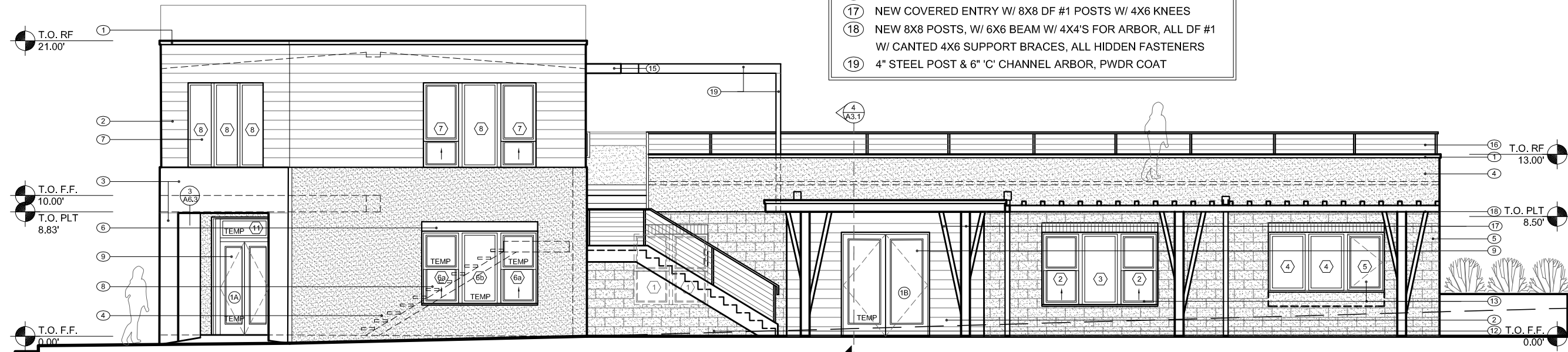
WEST ELEVATION
